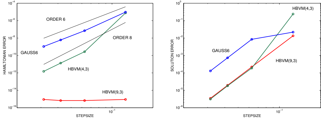
Figure 1: Kepler problem, e = 0.6 ; Hamiltonian (left plot) and solution (right plot) errors over 1000 periods with a constant stepsize.
