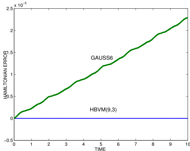
Figure 5: restricted three-body problem, orbit starting at (25); Hamiltonian error when using tol = 10^{-10} and h_0 = 10^{-5} .
