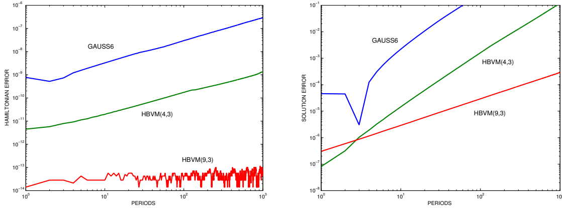
Figure 2: Kepler problem, e = 0.99 ; Hamiltonian (left plot) and solution (right plot) errors over 1000 periods with a variable stepsize, tol = 10^{-12} . Note that HBVM(4,3) is not energy preserving, on the contrary of HBVM(9,3).
