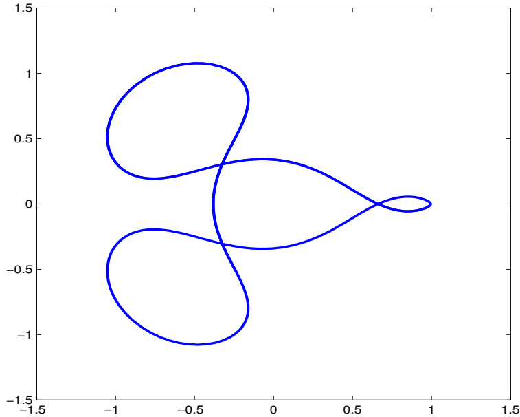
Figure 3: restricted three-body problem, Arenstorf's orbit corresponding to (24).
