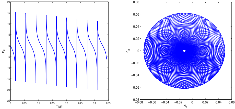
Figure 4: restricted three-body problem, orbit starting at (25).
