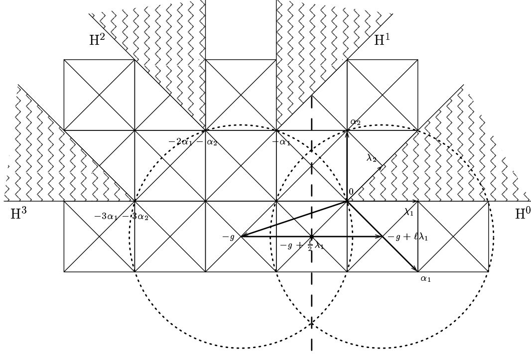
FIGURE 2. Twisting weights of \Omega^q over Q_3 by \mathcal{O}(\ell)
